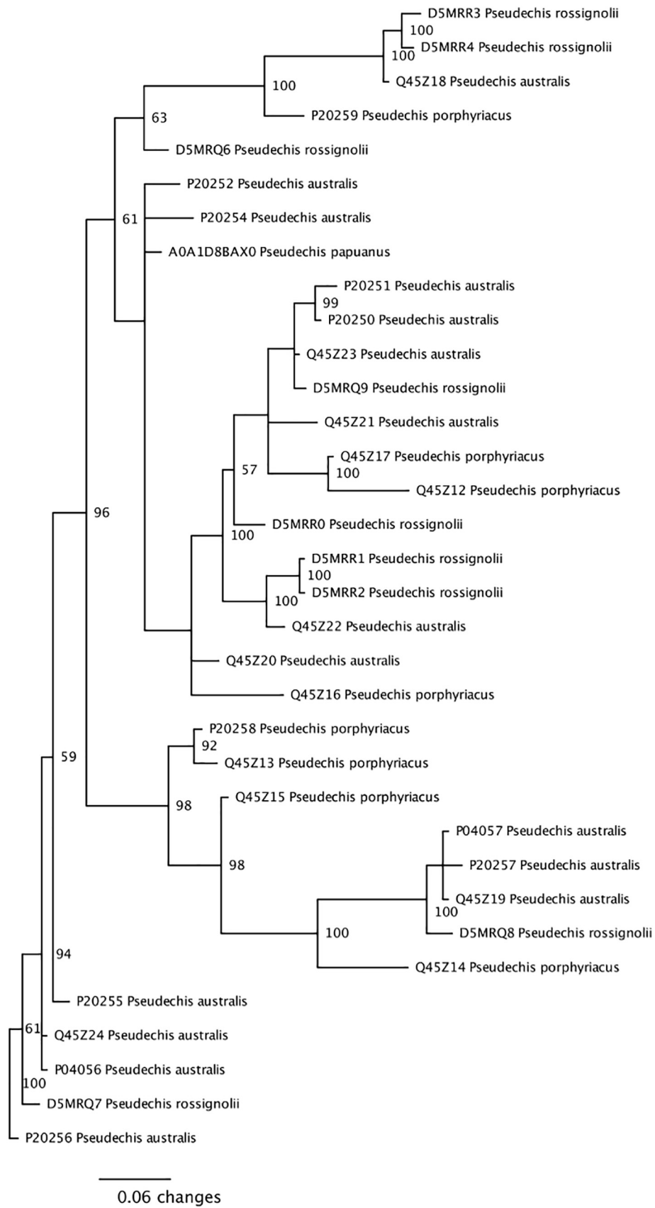
Fig. 3. Phylogenetics of the Pseudechis -specific clade of PLA 2 toxins. Notechis scutatus PLA 2 outgroup is not shown. Node values indicate posterior probabilities.
